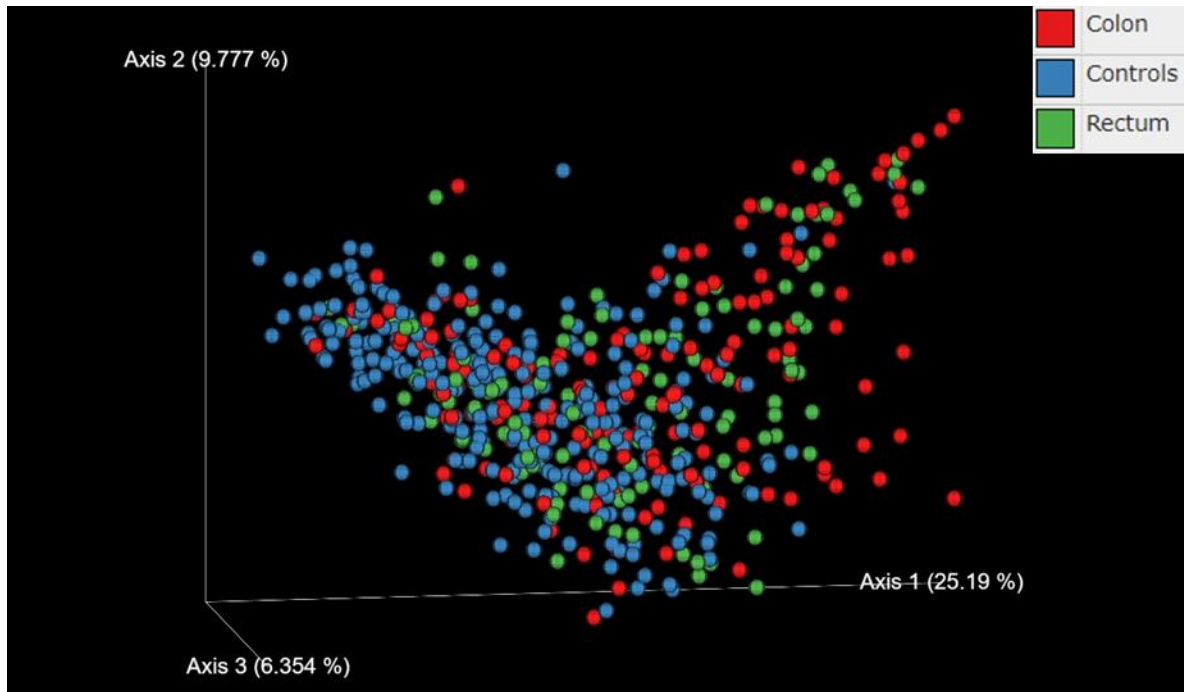
S2 Fig. Principal coordinate analysis plot of the weighted UniFrac distance based on anatomical sites.
