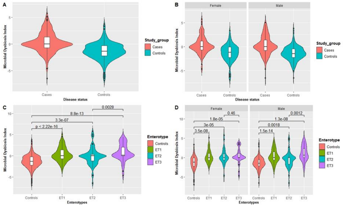
S10 Fig. Comparison of microbial dysbiosis index between colorectal cancer (CRC) cases and controls. (A) Total population. (B) Each sex. (C) Across enterotype-specific CRC cases. (D) Across enterotype-specific CRC cases by sex.
