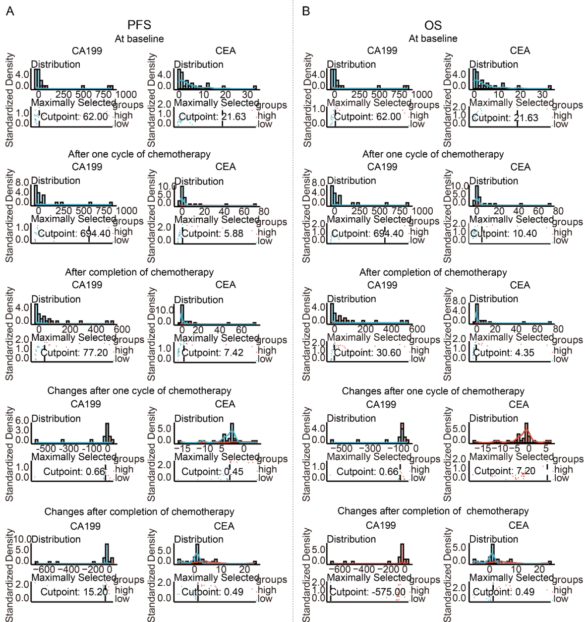
S6 Fig. The optimal cutoff values of tumor markers. (A) Optimal cutoff values for carbohydrate antigen (CA) 19-9 and carcinoembryonic antigen (CEA) associated with progression-free survival at baseline, post-treatment and their changes after treatment. (B) Optimal cutoff values for CA19-9 and CEA associated with overall survival at baseline, post-treatment and their changes after treatment.
