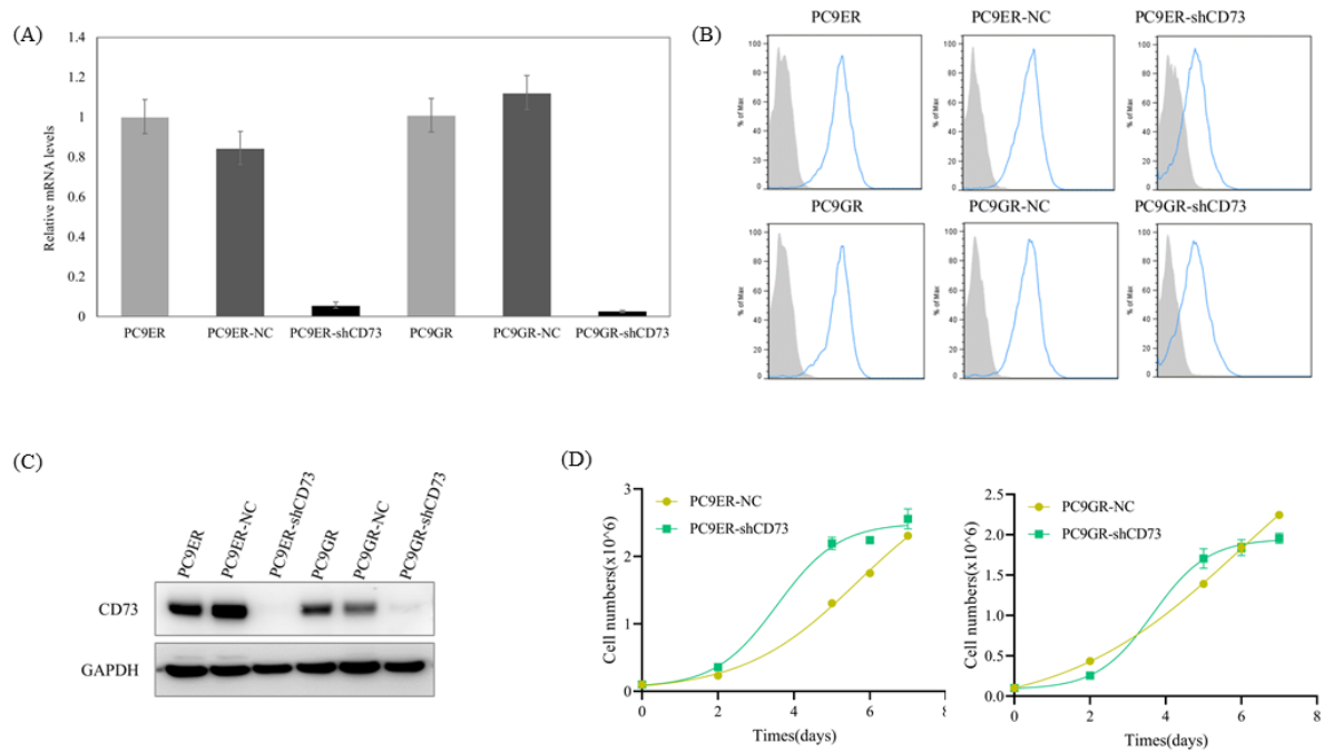
S1 Fig. Characteristics of the shCD73 transduced lung cancer cell lines. (A) The mRNA expressions of CD73 in each cell line. CD73 protein expression was assessed by (B) flow cytometry and (C) immunoblot assay. (D) The proliferation of PC9ER and PC9GR cells transduced with lentivirus containing shRNA CD73.
