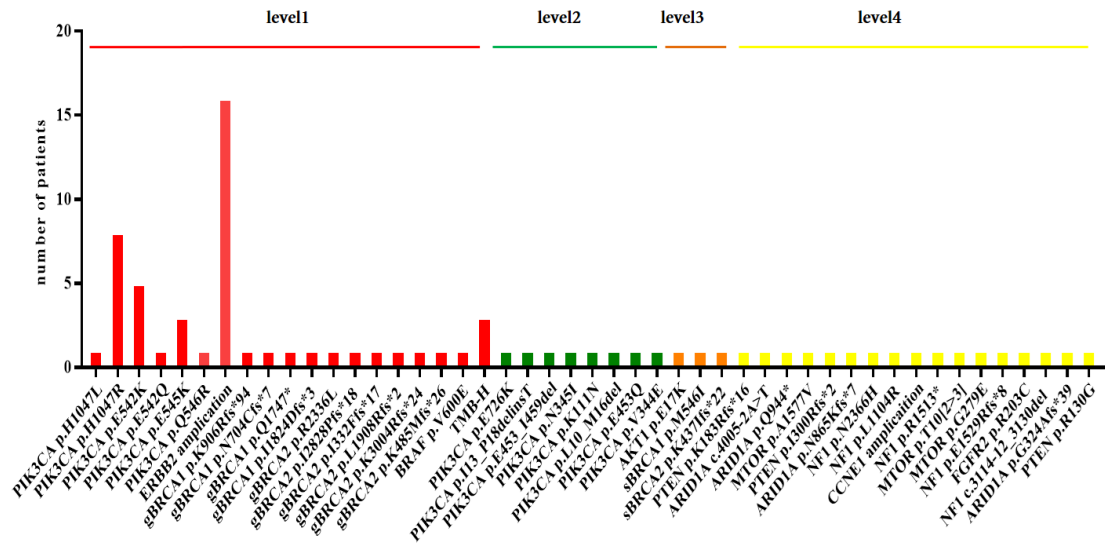
S9 Fig. The number of patients with undetectable molecular residual disease (MRD) in different actionable alterations. gBRCA1, germline BRCA1 mutation; gBRCA2, germline BRCA2 mutation; sBRCA1, somatic BRCA1 mutation; sBRCA2, somatic BRCA2 mutation; TMB-H, TMB-high.
