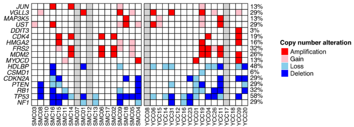
S14 Fig. The landscape of ploidy-based copy number variations in this study cohort. Sample order of this landscape is the same with that of Fig. 1. Classification of copy number variations is described in Supplementary Methods.
