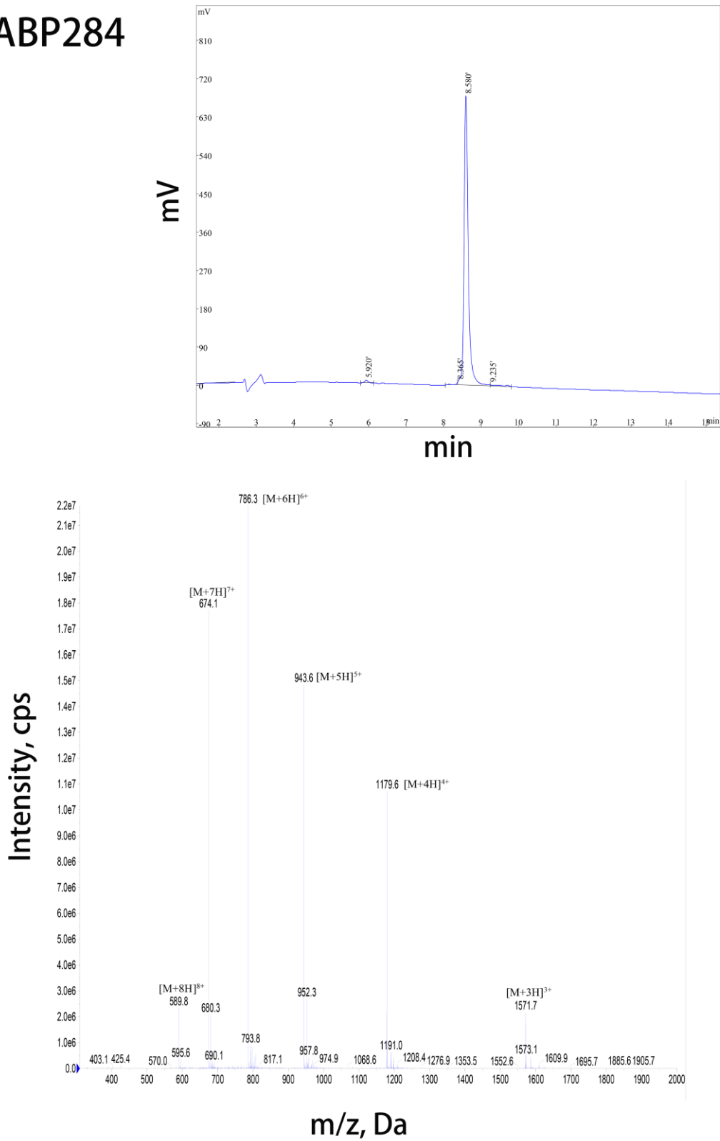
S1 Fig. The electrospray ionization mass spectrometry/high-performance liquid chromatography results of nABP284.
