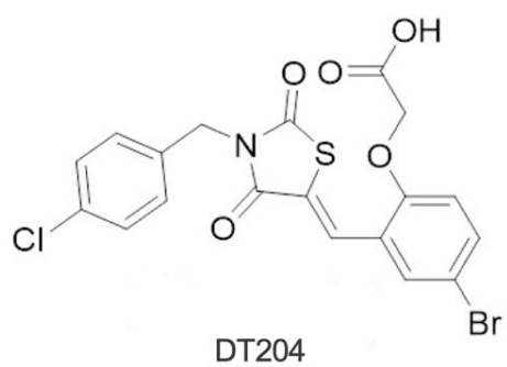
S16 Fig. The chemical structures of DT204 and SZLP1-41. The chemical structures of DT204 and SZLP1-41 were shown.
