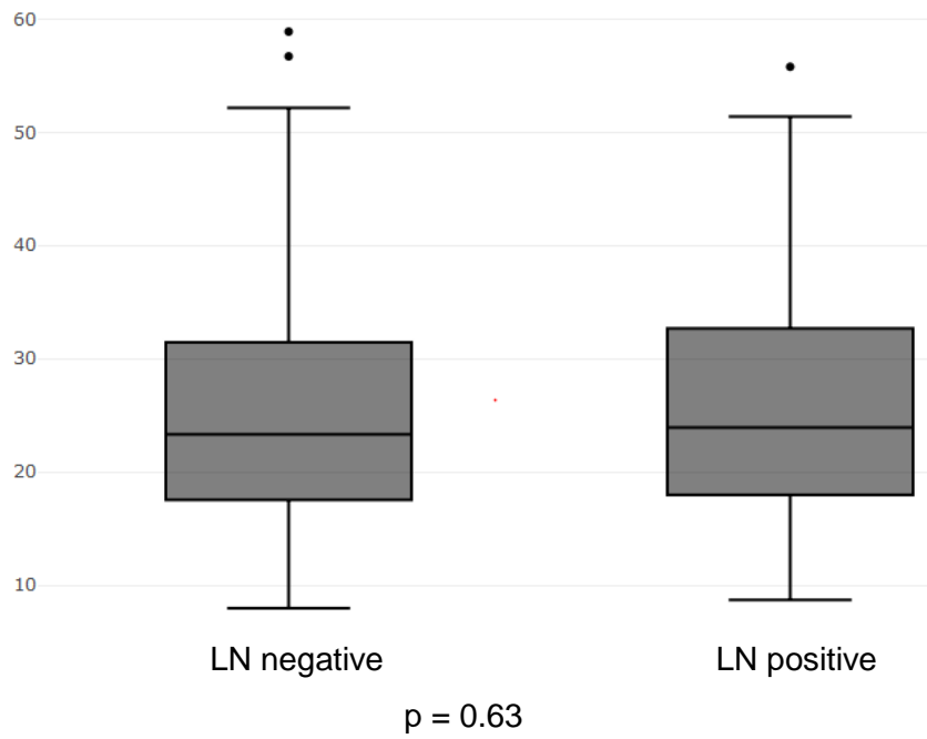
S6 Fig. Distribution of immunoscore-like score according to the lymph node (LN) metastasis in the overall set (n=316).
