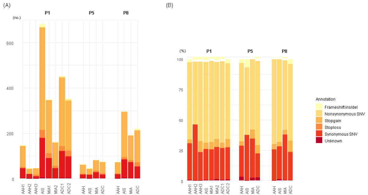
S3 Fig. Distribution of mutation according to the exonic function frequency (A) and proportion (B). AAH, atypical adenomatous hyperplasia; ADC, adenocarcinoma; AIS, adenocarcinoma in situ ; MIA, minimally invasive adenocarcinoma; VAF, variant allele frequency.
