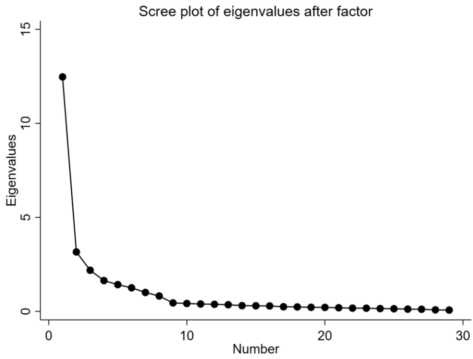
S1 Fig. Scree plot for principal component analysis.
