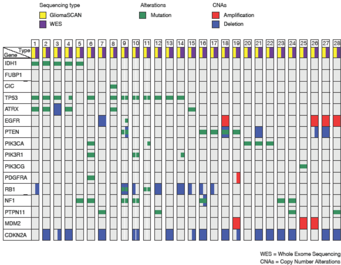
S9 Fig. Comparing with somatic alterations using whole exome sequencing and GliomaSCAN.
