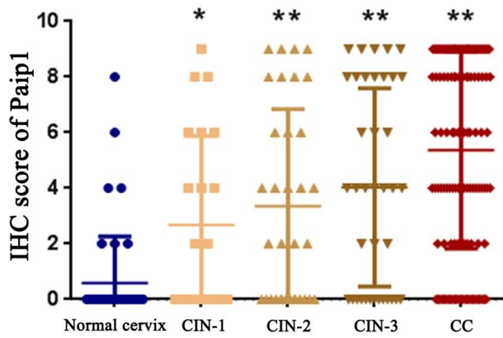
S1 Fig. Poly(A)-binding protein-interacting protein 1 (Paip1) expression was significantly up-regulated in cervical cancer (CC). Quantification of Paip1 expression levels in the tissues detected by immunohistochemistry (IHC). CIN, cervical intraepithelial neoplasia.
