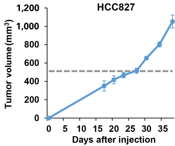
S2 Fig. Tumor growth curves of various tumor models. Data represent means \pm standard error of mean ( n \geq 8 ).
